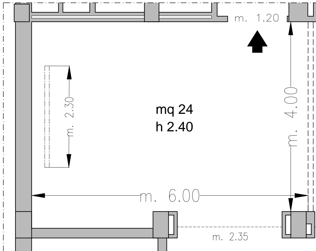
Piano -1 / Basement
